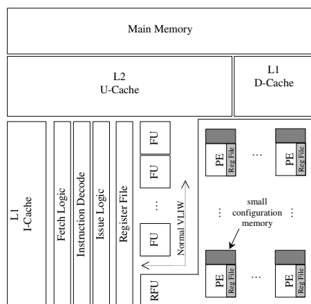
Figure 1 Example CRISP instance
