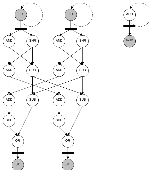
Figure 3 Data dependence graph with intercluster transfers shown as a thick line.
